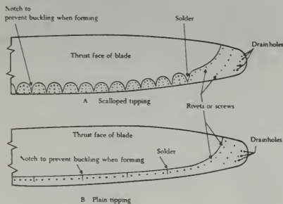
FIGURE 7-8. Installation of metal sheath and tipping.
